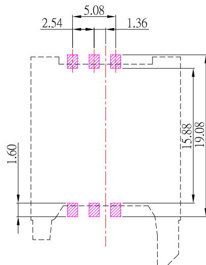
P.C.B LAYOUT MOUNTING PATTERN TOP VIEW
