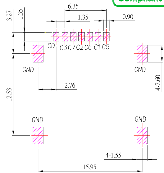
PCB LAYOYT
