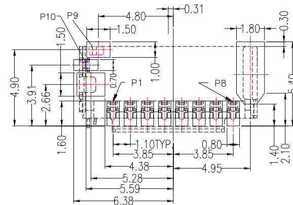
PCB LAYOYT
