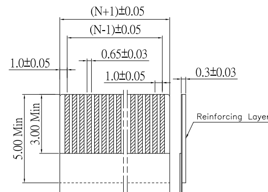
RECOMMENDED FFC/FPC DIM.
