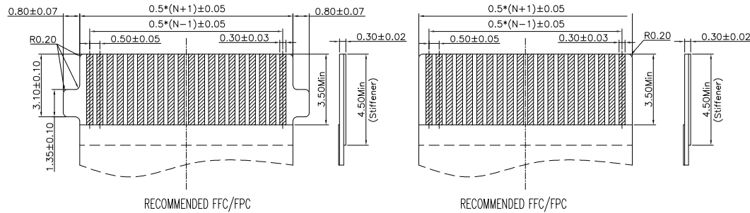
RECOMMENDED FFC/FPC
