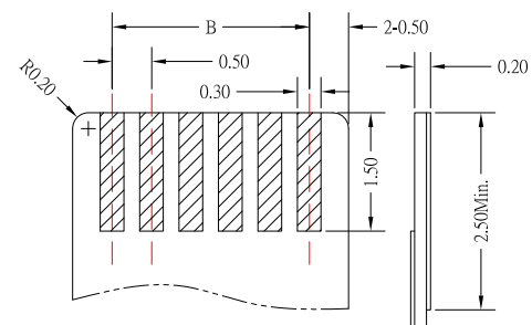
APPLICABLE FFC/FPC
