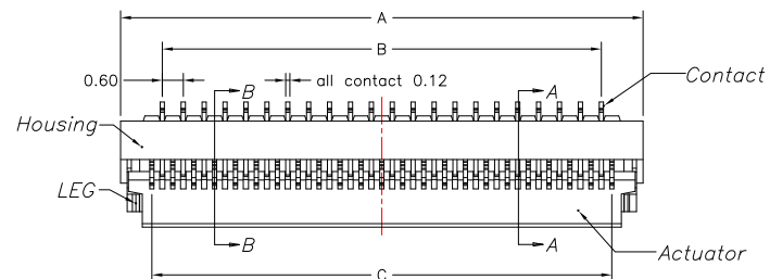
When Actuator Is Opened Scale 2:1
