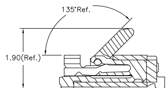
When Actuator Is Opened Scale 2:1
