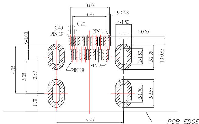
RECOMMENDED PCB LAYOUT THICKNESS TOP VIEW
