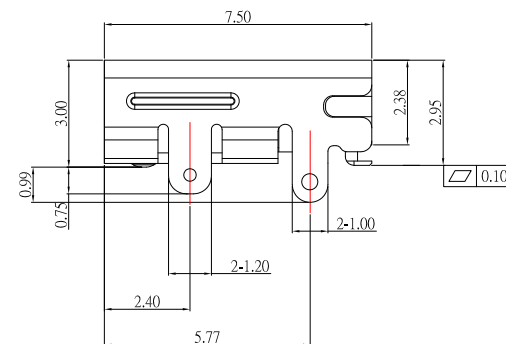
RECOMMENDED PCB LAYOUT THICKNESS TOP VIEW
