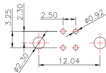
P.C.B LAYOUT MOUNTING PATTERN
