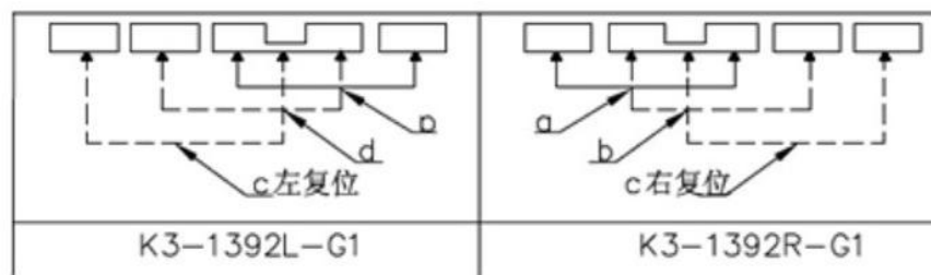
Schematic(Shorting)
