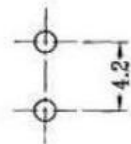
P.C.B LAYOUT BOTTOM VIEW
