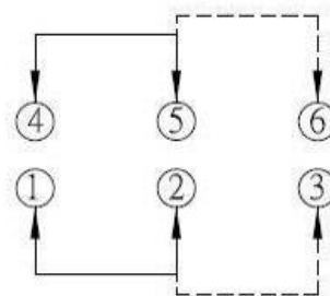
SCHEMATIC (NON-SHORTING)
