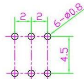
P.C.B LAYOUT MOUNTING PATTERN
