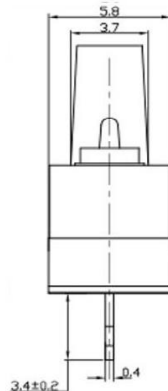
SCHEMATIC (NON-SHORTING)
