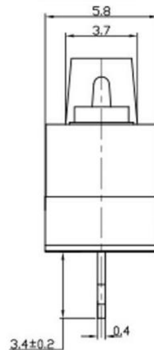
SCHEMATIC (NON-SHORTING)
