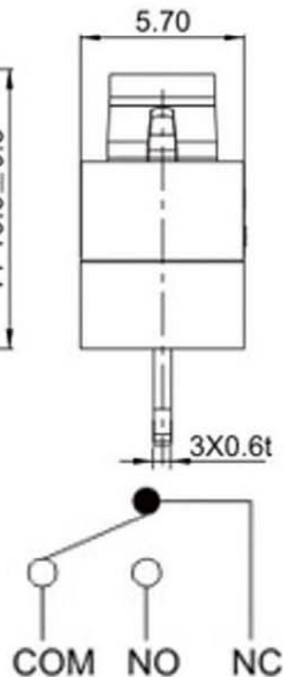
Circuit Diagram
