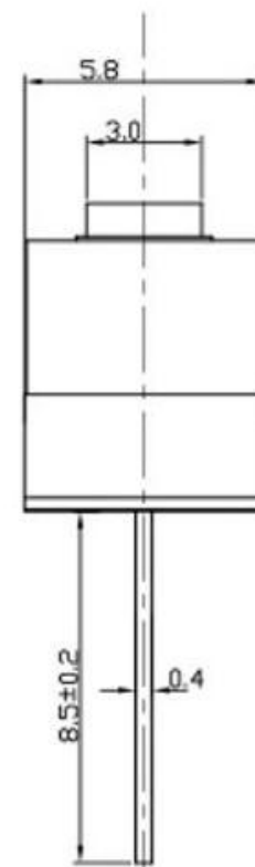
SCHEMATIC (NON-SHORTING)
