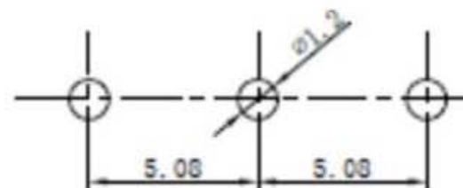
P. C. B HOLE
