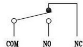
SCHEMATIC (NON-SHORTING)
