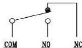
SCHEMATIC (NON-SHORTING)
