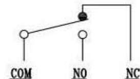
SCHEMATIC (NON-SHORTING)
