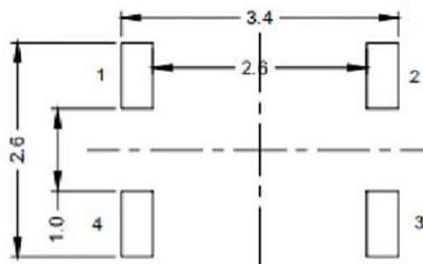
PCB layout
