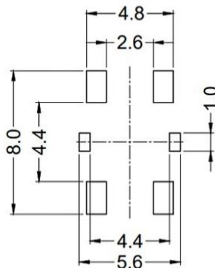
PCB layout
