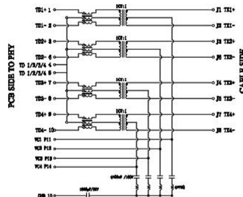
SCHEMATIC
