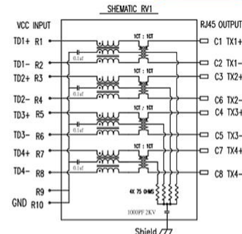
SCHEMATIC
