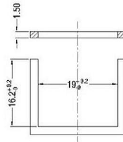
PANLE CUT-OUT
