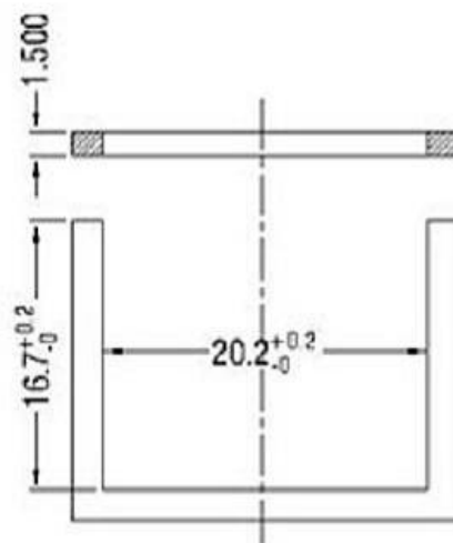
PANEL CUT-OUT
