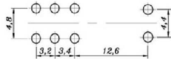
PCB LAYOUT
