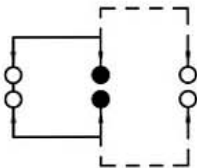
SCHEMATIC (NON-SHORTING)
