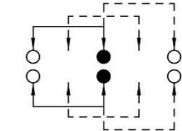
SCHEMATIC (NON-SHORTING)
