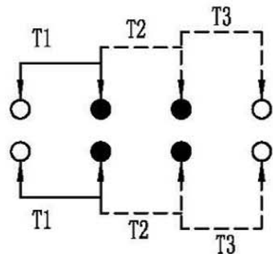
SCHEMATIC (NON-SHORTING)
