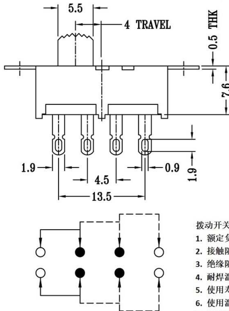
SCHEMATIC (NON-SHORTING)
