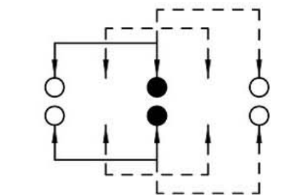
SCHEMATIC (NON-SHORTING)
