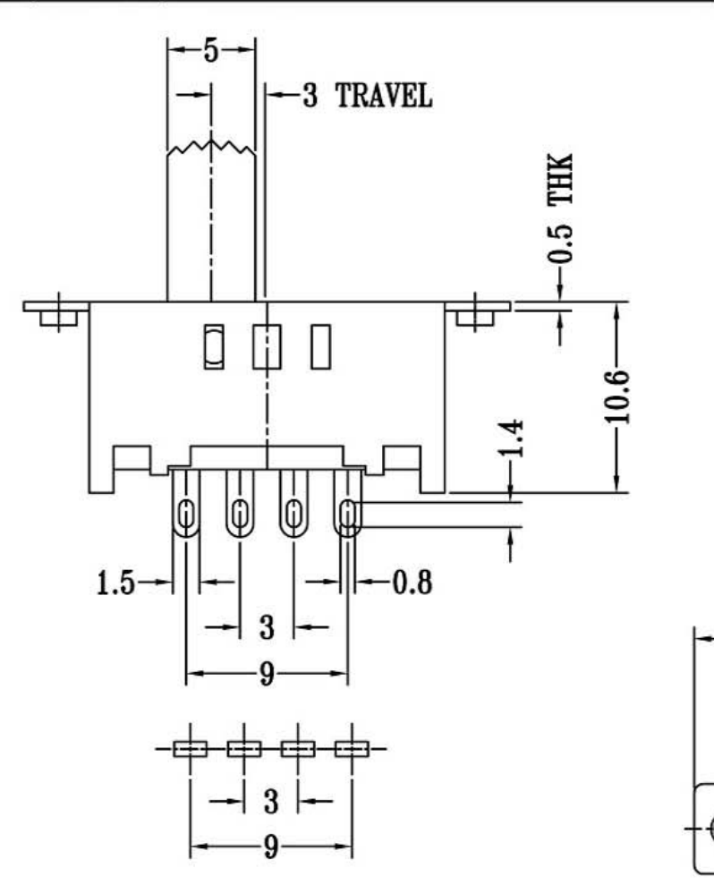
P.C.B LAYOUT BOTTOM VIEW
