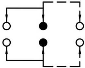
SCHEMATIC (NON-SHORTING)
