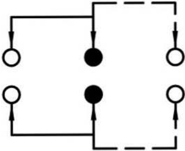
SCHEMATIC (NON-SHORTING)
