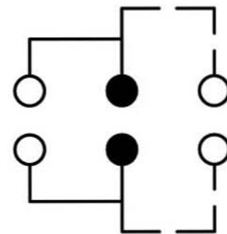
SCHEMATIC (NON-SHORTING)
