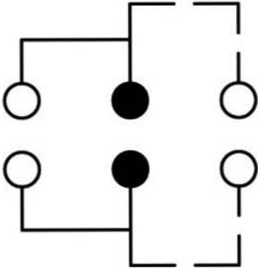
SCHEMATIC (NON-SHORTING)
