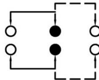
SCHEMATIC (NON-SHORTING)
