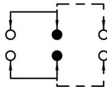
SCHEMATIC (NON-SHORTING)
