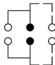
SCHEMATIC (NON-SHORTING)
