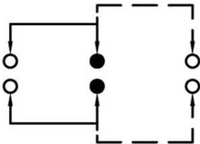
SCHEMATIC (NON-SHORTING)
