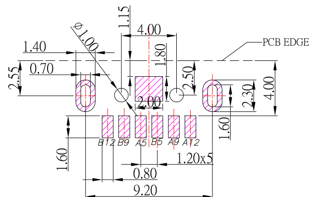
P.C.B LAYOUT MOUNTING PATTERN
