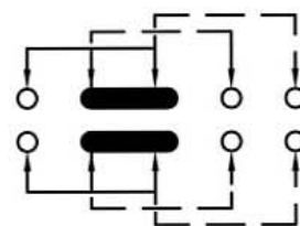
SCHEMATIC (SHORTING)
