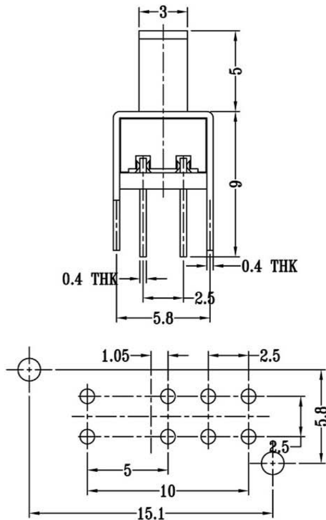
P.C.B LAYOUT BOTTOM VIEW
