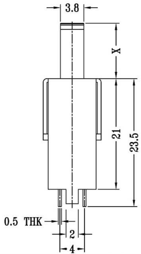
SCHEMATIC (SHOTRING)
