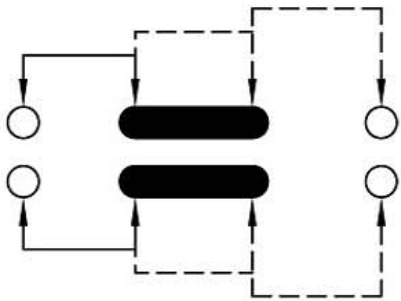
SCHEMATIC (NON-SHORTING)
