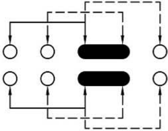
SCHEMATIC (SHORTING)
