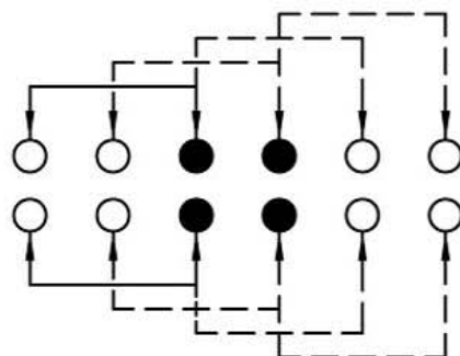
SCHEMATIC (SHORTING)
