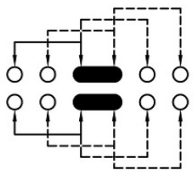
SCHEMATIC (SHORTING)
