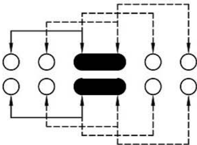
SCHEMATIC (SHORTING)
