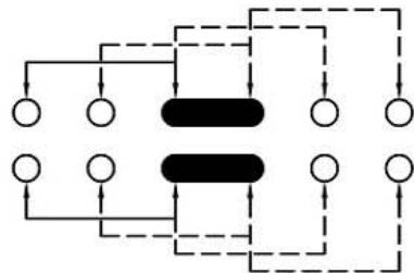
SCHEMATIC (SHORTING)
